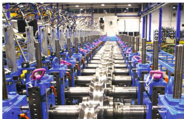
Roll forming
